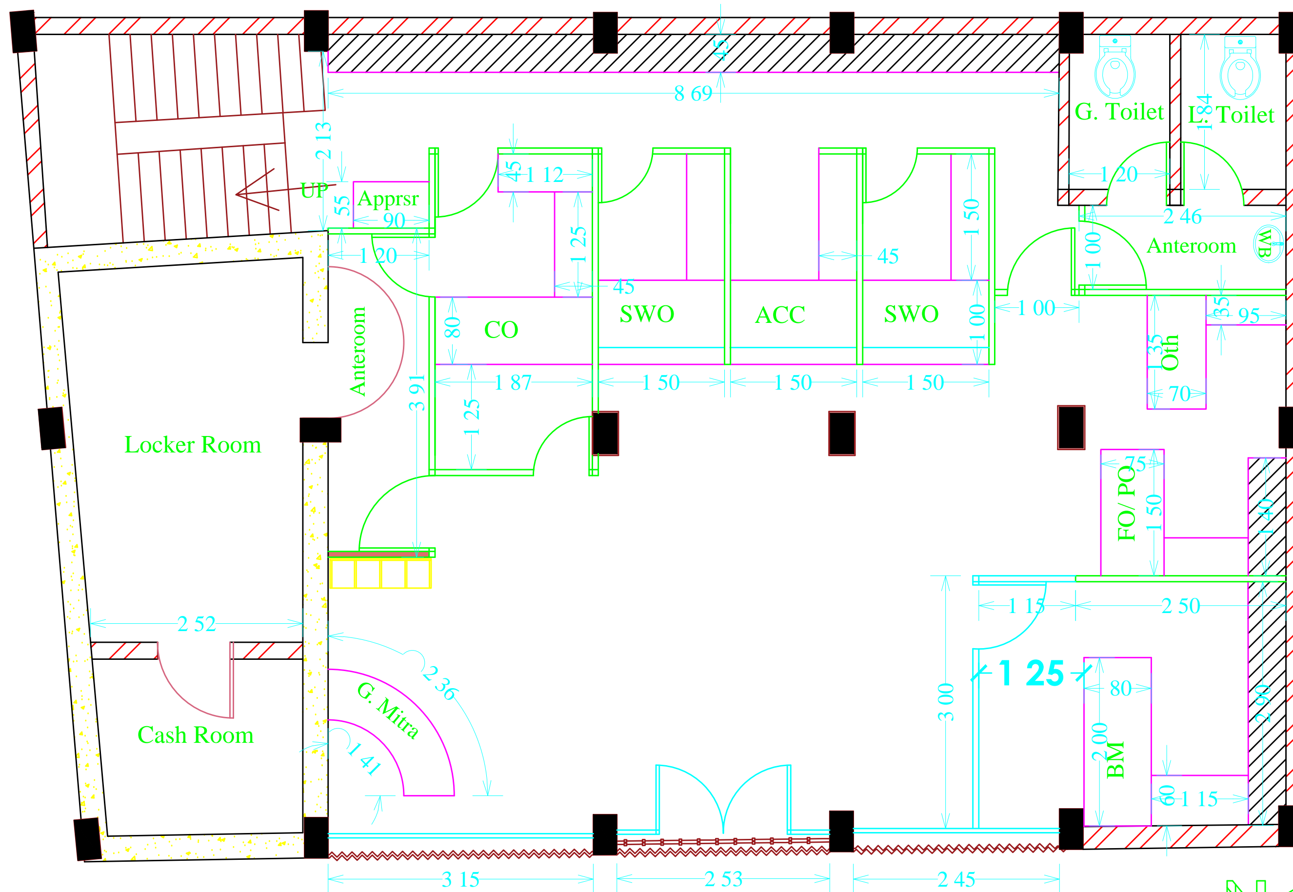
SBI CHERUTHURUTHY BRANCH - PROPOSED GF LAYOUT
